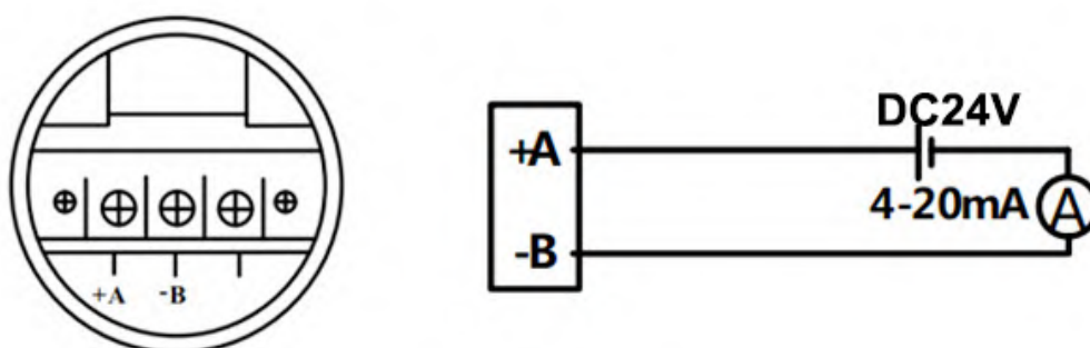
4-20 mA Output
